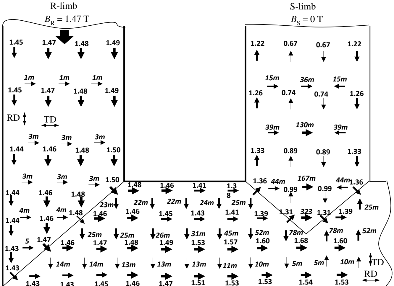
Fig.4. Local instantaneous distribution of induction values B_{RD} , B_{TD} and B_{DD} , for the time instant of zero flux in the middle S-limb, assuming four main flux paths (4FP). All induction values B_{RD} and B_{DD} are given in T, values B_{TD} in mT.
