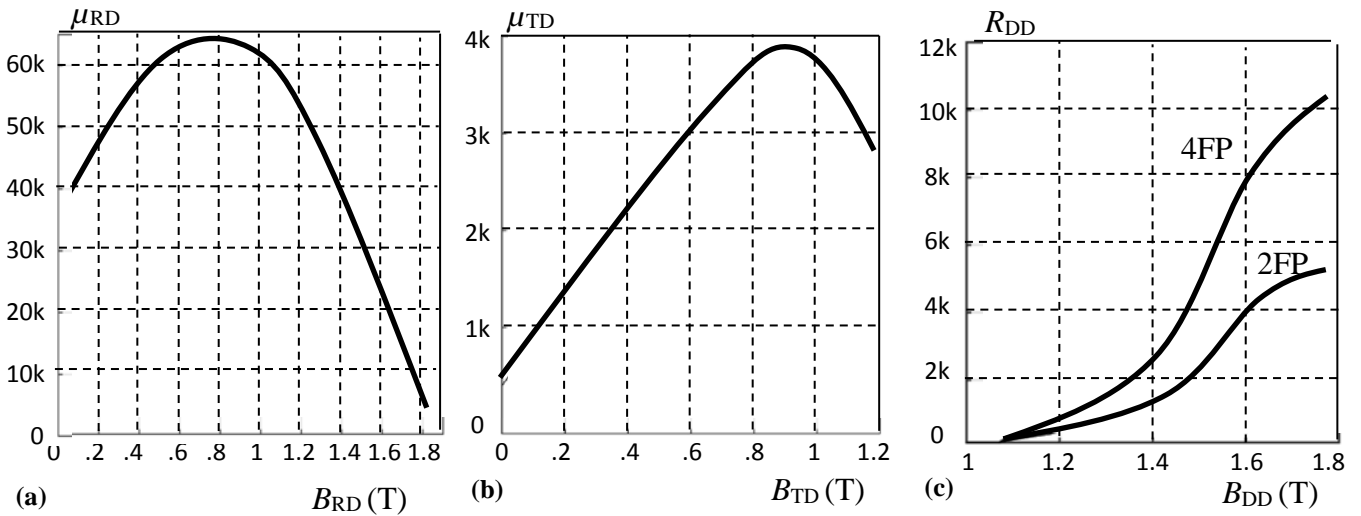
Fig.2. Data of the investigated electrical steel 23ZDKH95. (a) Relative permeability \mu_{RD} in rolling direction, as a function of the induction B_{RD} [9]. (b) \mu_{TD} in transverse direction, as a function of B_{TD} [9]. (c) Overlap reluctances R_{DD} as a function of the induction B_{DD} for two-path modelling and four-path modelling, respectively (roughly estimated from [10]).
