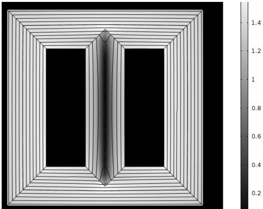
Fig.6. Comparison result as attained from FEM modelling of high resolution, however neglecting effects of overlap regions in corners and T-joints. Differences of local induction are coded by
