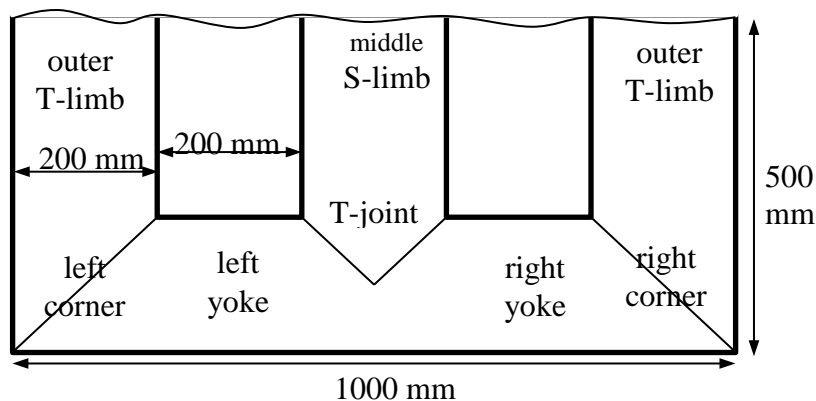
Fig. 1. The modelled lower half of the investigated 3-phase, 3-limb transformer core package.
