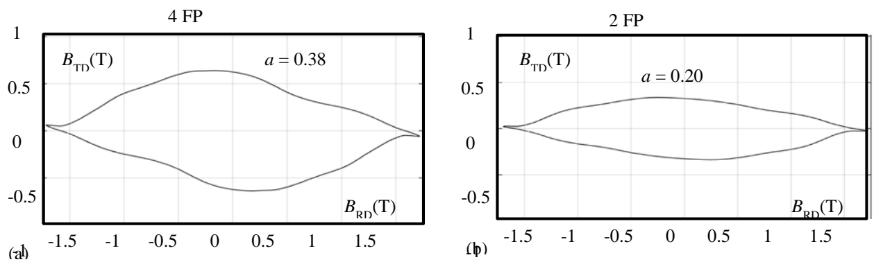
Fig.5. Vector magnetization patterns \mathbf{B}(t) for the region of V-end of the S-limb laminations.
